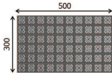
300x500x6T
